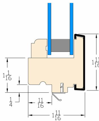
Sill Rail Detail
